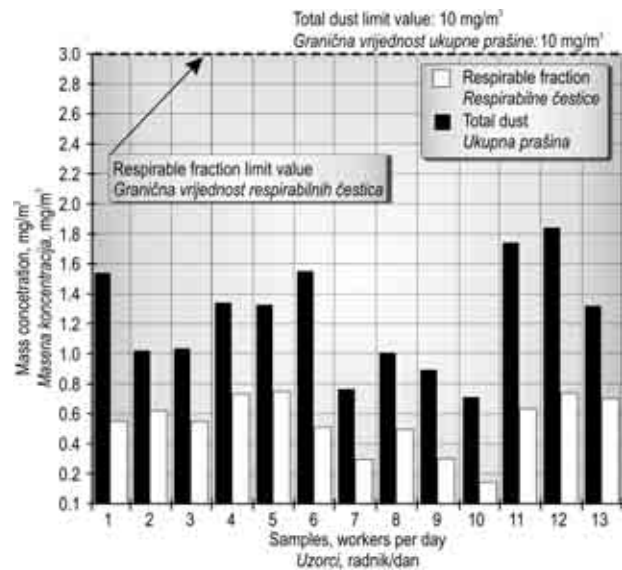
Figure 4. Comparison between the obtained mass concentrations of respirable particles/total dust and maximum permissible concentrations (limit values)
