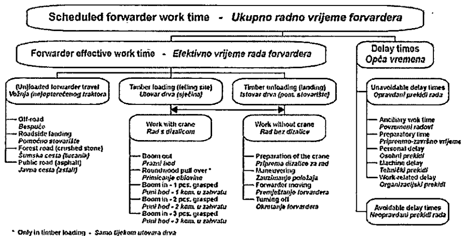
Figure 3. Working components
