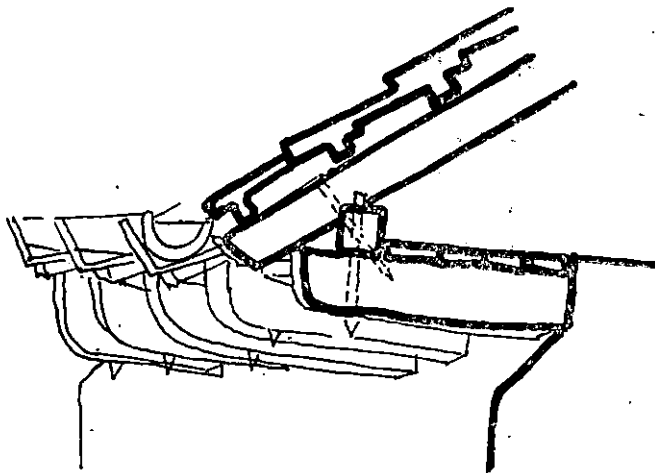
Sl. — Fig. 10. Skica konstrukcije krova — Schematic diagram of a roof construction.
