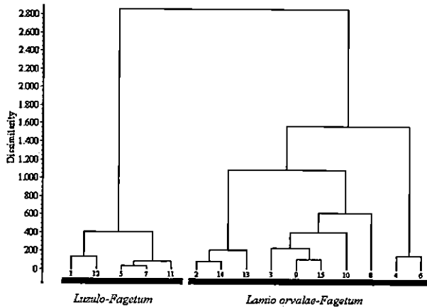
Figure 2 Dendrogram constructed by cluster analysis - Incremental sum of squares. Slika 2 Dendrogram izrađen klusterskom analizom - Incremental sum of squares.
