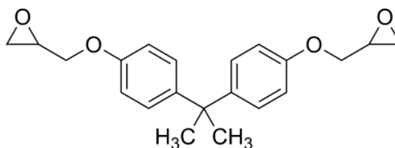
Slika 16. Bisfenol-A-diglicidiletera (Wikipedia, 2023)
